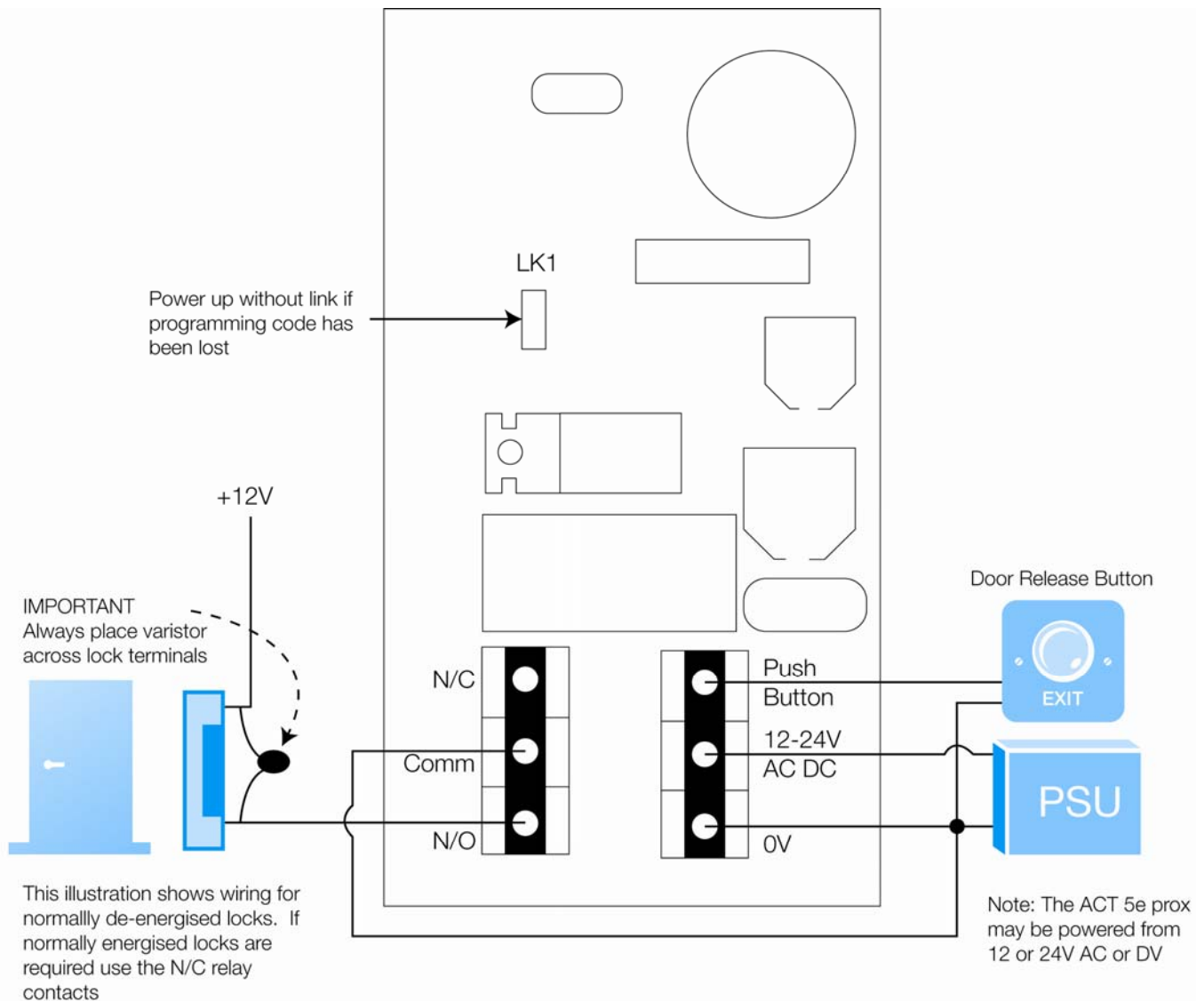
Figure 1: ACT 5e prox Wiring Diagram for Strike Lock
